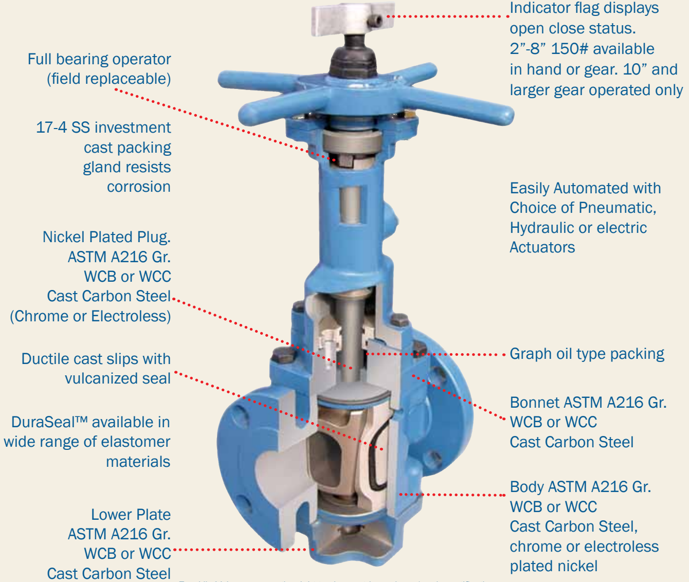
MANUAL BLEED
