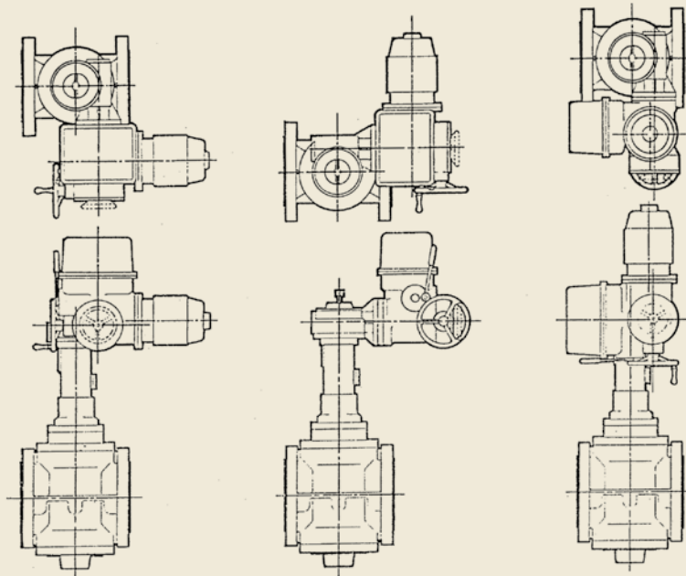
STYLE "A" - (Standard mounting) MOTOR OPERATOR MOUNTED PARALLEL TO PIPE LINE
