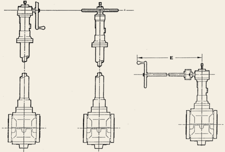
GEAR OPERATOR EXTENSION-CLOSED TYPE "A"
